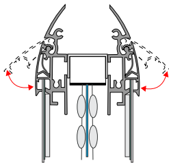
Double Sided LED Illumination
