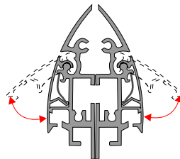
Double Sided No Illumination
